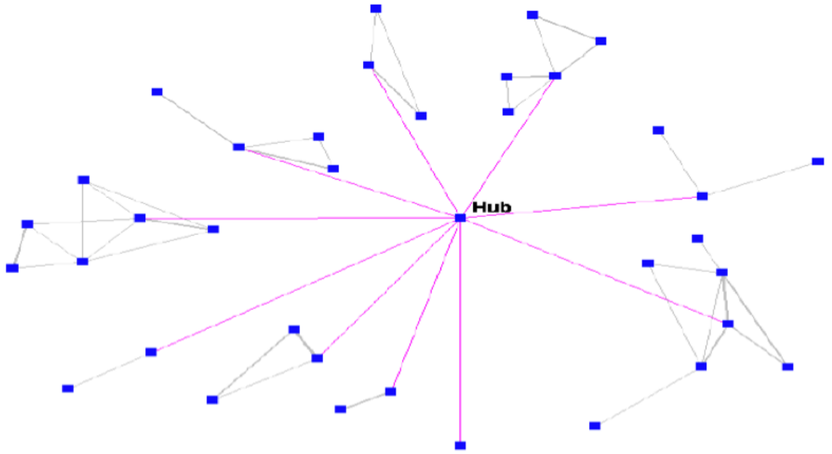
Figure 2 – Hub-and-Spoke Network
